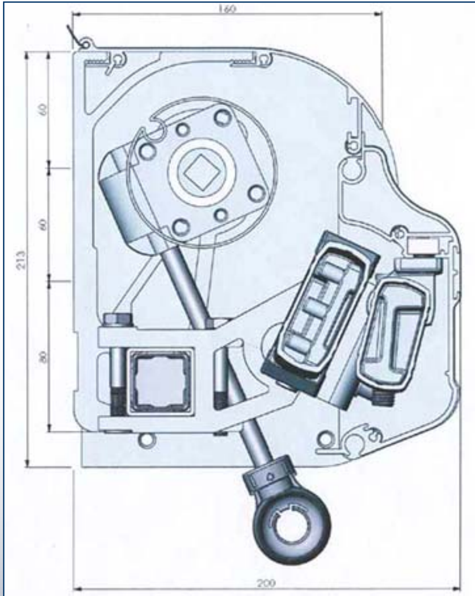
Image showing section through end of SENATOR cassette box, illustrating winding mechanism and handle connector for manual operation.
