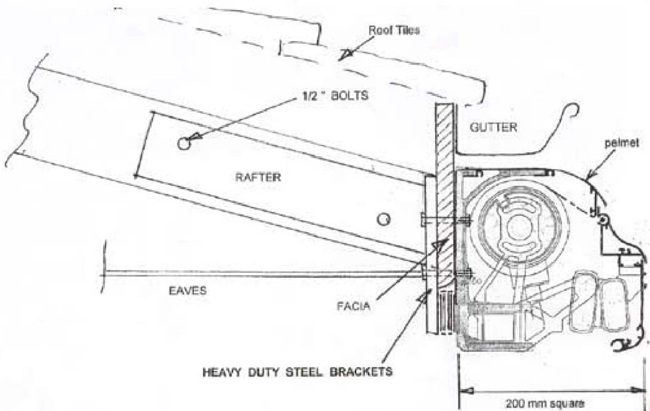
Image showing section through SENATOR cassette awning in fixed position.
