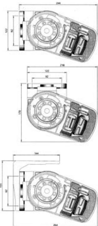
Image showing section through LINEA cassette awning motor box
